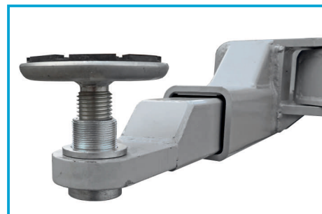
ADAPTERS WITH DOUBLE ADJUSTABLE THREAD
